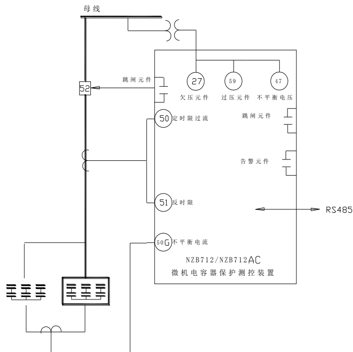
图 1 NZB7121/NZB7121AC/NZB7122/NZB7122AC/NZB7128/NZB7128AC 功能配置图
