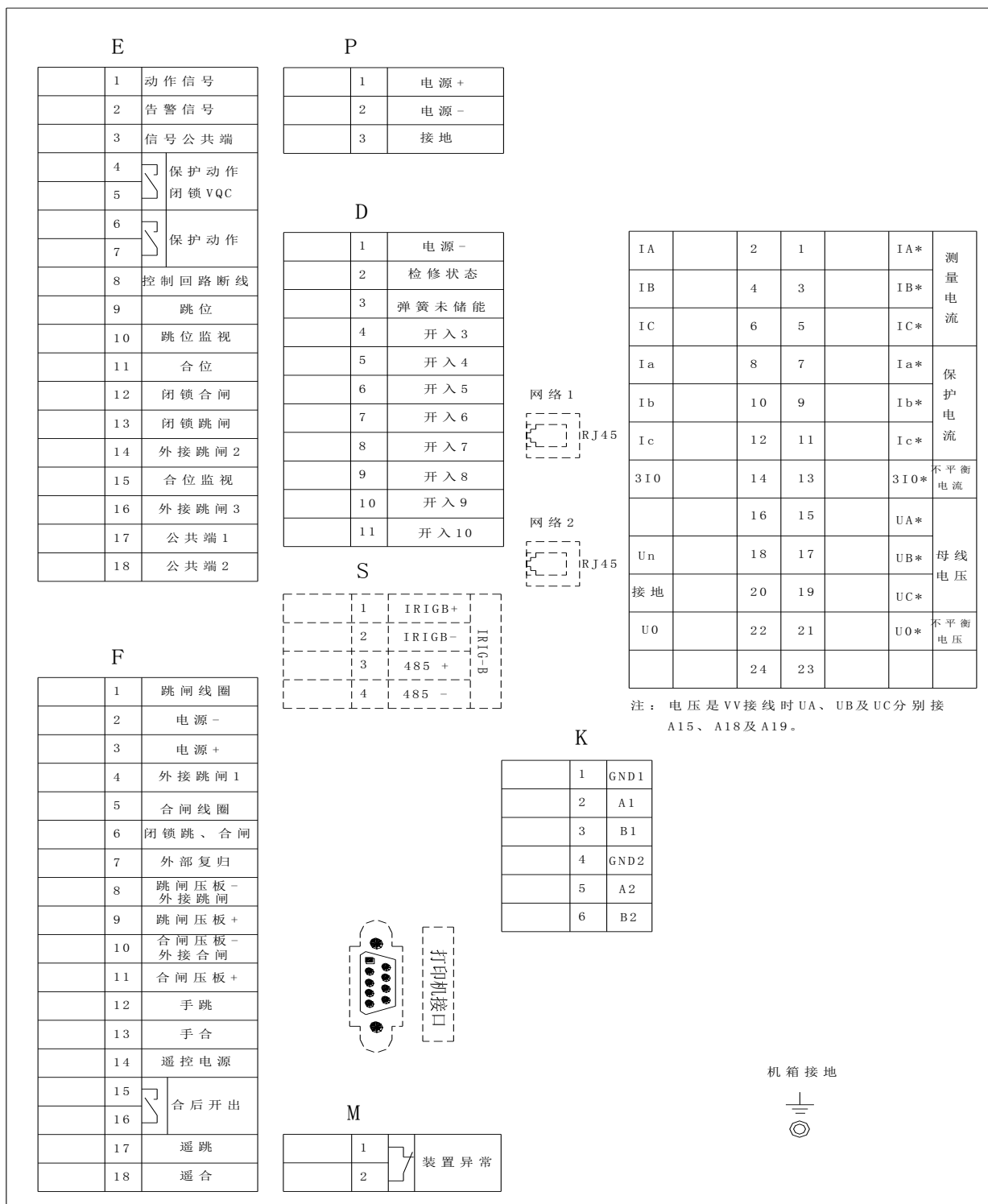
图 5 NZB7121DC/AC/ NZB7122DC/AC NZB7123DC/AC 端子图
